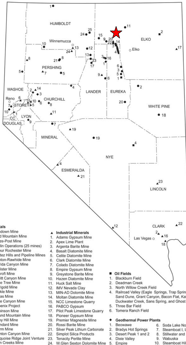
Major mines, oil fields, and geothermal plants, 2008.
